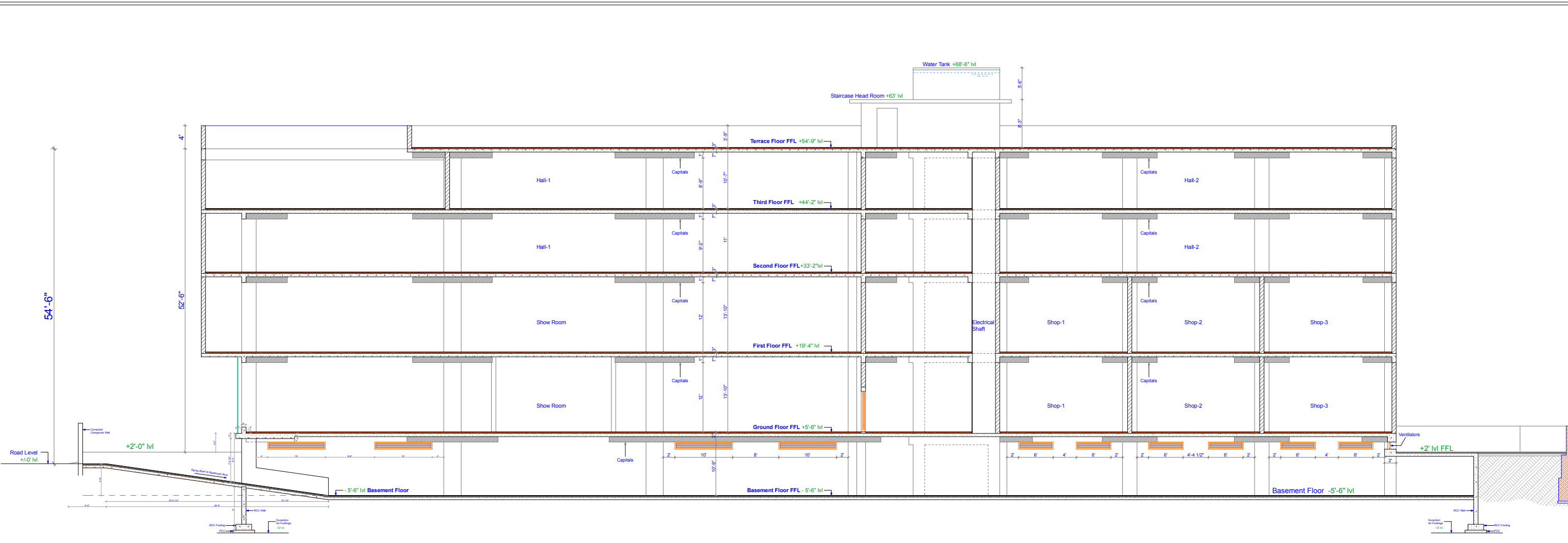
SECTION AT 'Y-Y' Date : 13th February 2020
